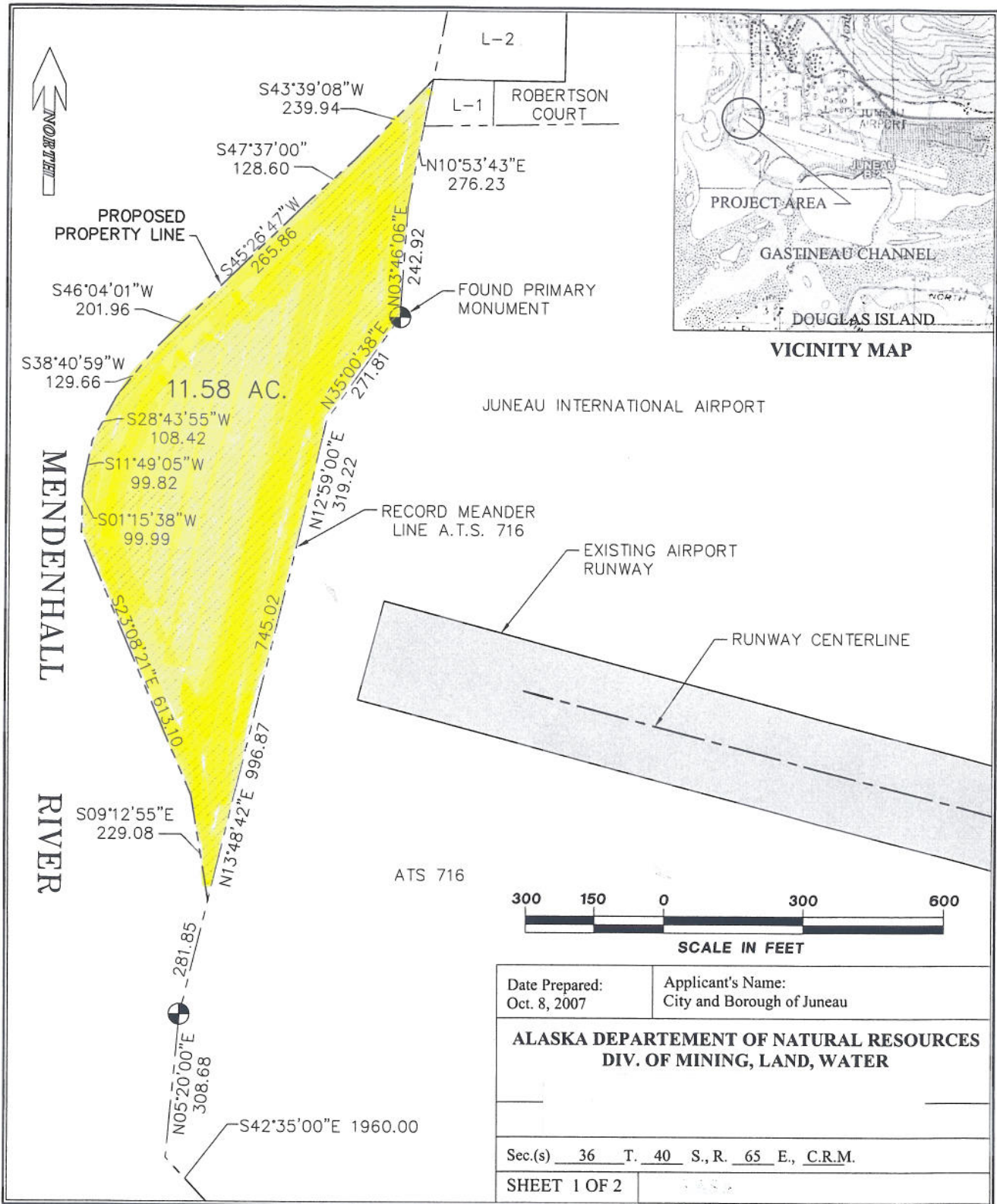
Attachment 'A' - ADL 107380 Conveyance Diagram Parcel #2
